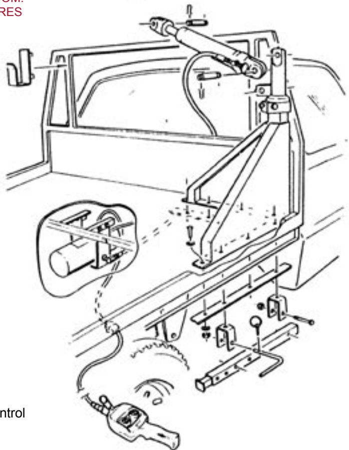
SHOWN HERE IS A TYPICAL INSTALLATION MODEL L-12RLP LINDELL HOIST
